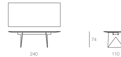
B26A table with central section
