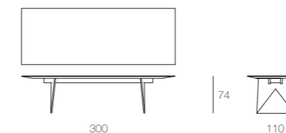
B26C table with central section
